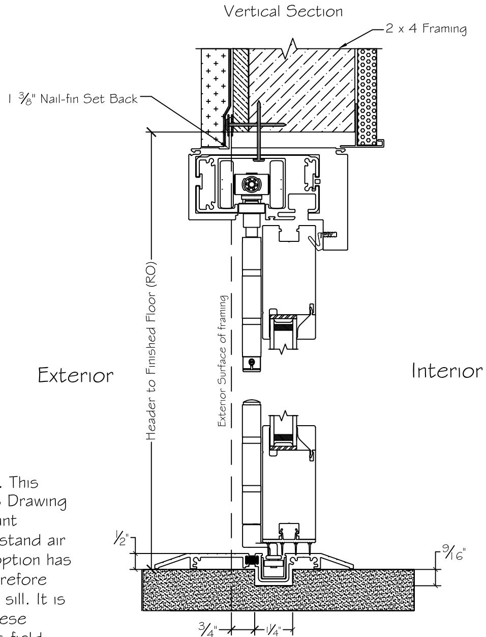
The exterior edge of the 1\frac{1}{4} " groove is \frac{3}{4} " from the exterior edge of the framing.
