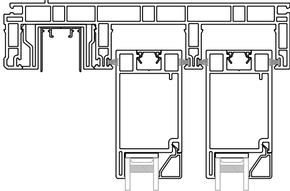
Vertical Section View
