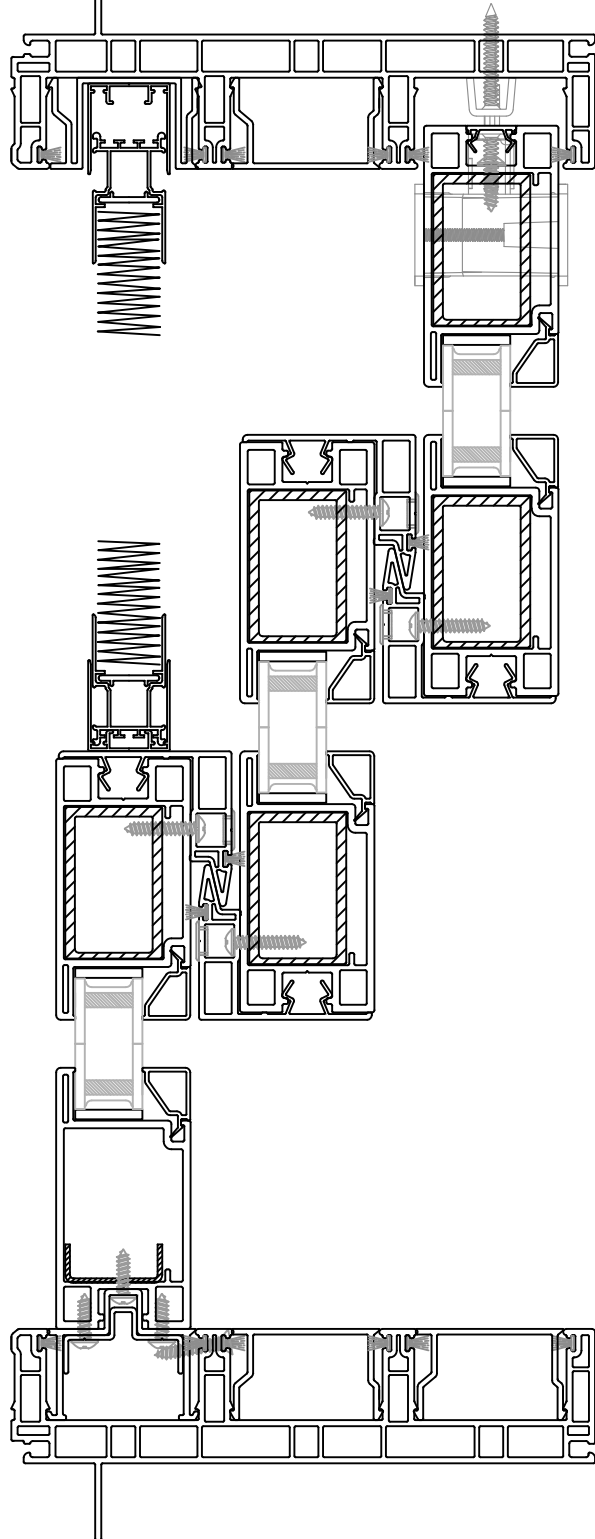
Horizontal Section View
